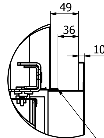
C (1:4)
